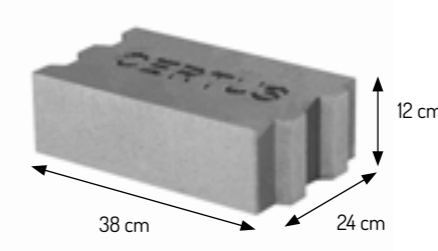
Bloczek P+W
