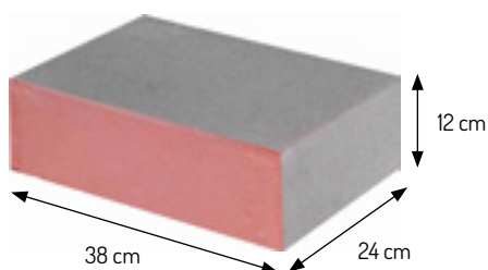
Bloczek BF01
