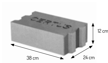
Bloczek P+W
